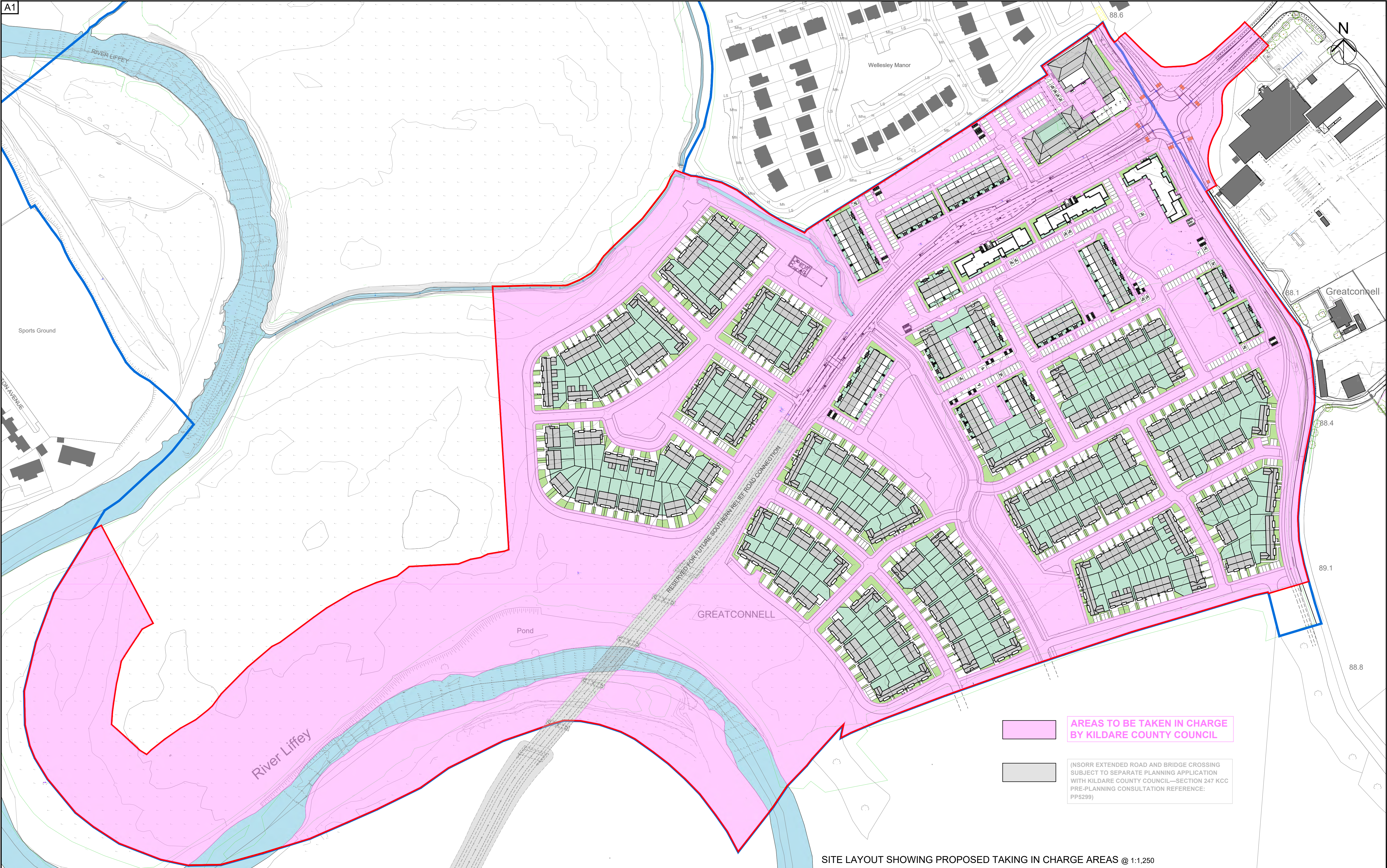
SITE LAYOUT SHOWING PROPOSED TAKING IN CHARGE AREAS @ 1:1,250
